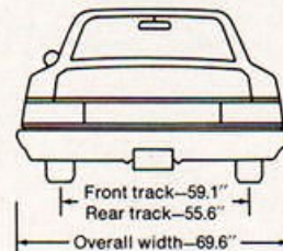
Plymouth Scamp 2-Door Hardtop
