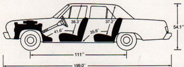
Plymouth Valiant 4-Door Sedan
