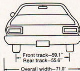
Plymouth Duster 2-Door Coupe
