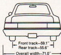
Plymouth Valiant 4-Door Sedan
