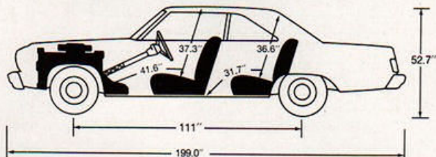
Plymouth Scamp 2-Door Hardtop
