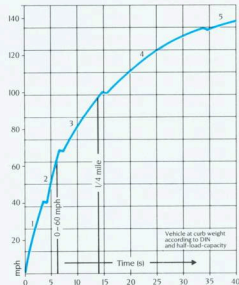
Acceleration Curve Manual gearbox
